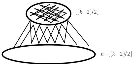
FIG. 2. An almost extremal graph for the Erdős-Sós conjecture.
