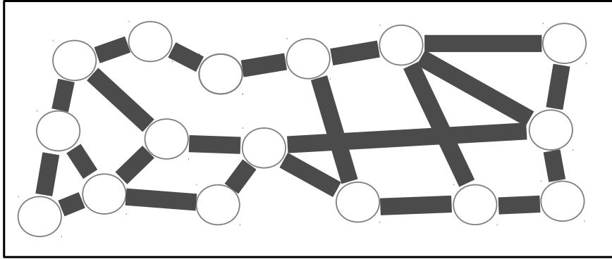
FIG. 4. A locally dense graph as in Lemma 2.5. The sets W_1, \dots, W_\ell are depicted with gray circles. Even though there are a large number of them, each W_i is linked to only boundedly many other W_j 's (at most four in this example). Lemma 2.5 allows us to regularize all the bipartite graphs using the same system of partitions of the sets W_i .
