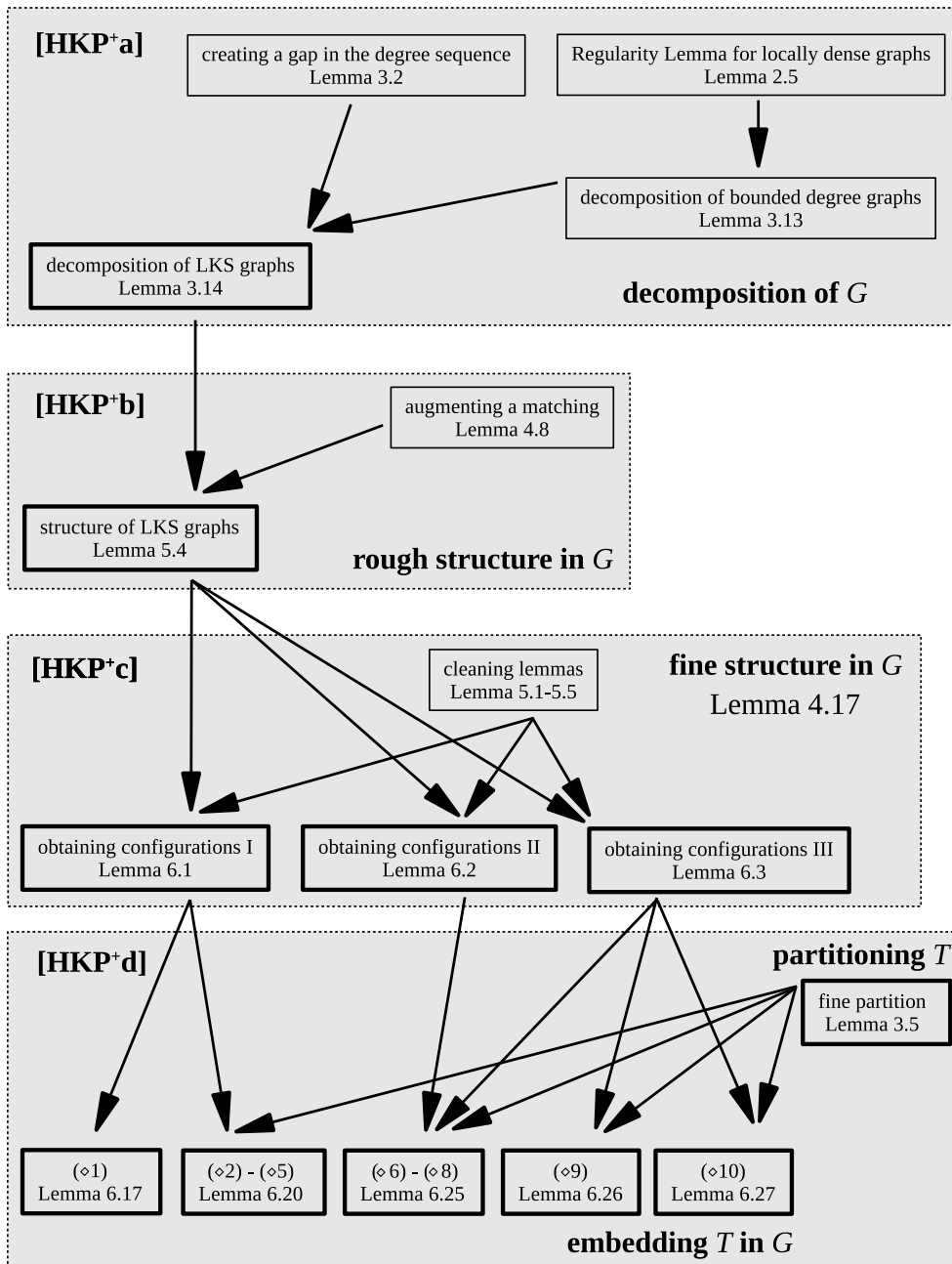
FIG. 3. Structure of the proof of Theorem 1.3, including parts from [HKP + b, HKP + c, HKP + d].
