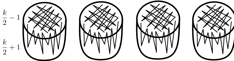
FIG. 1. An extremal graph for the Loebel-Komlós-Sós conjecture.
