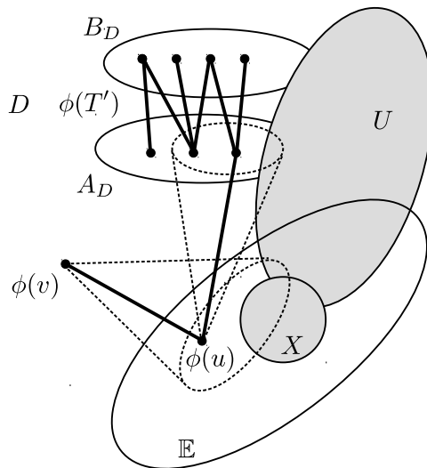
FIG. 5. Embedding using the set \mathbb{E} .
