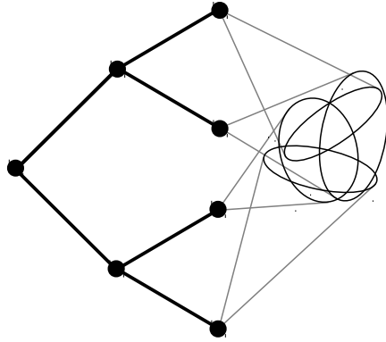
FIG. 6. Embedded part of the binary tree in bold. The neighborhoods of active vertices may overlap.
